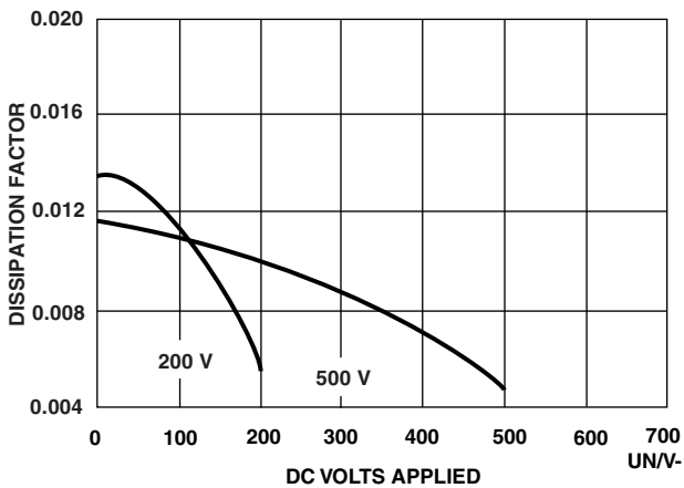
DISSIPATION FACTOR VS. VOLTAGE
