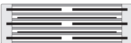
Extended foil design with internal series connection and metallized film (series connection of 2 elements)
